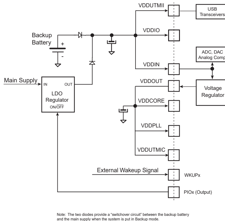
Figure 23-4. Battery Backup
