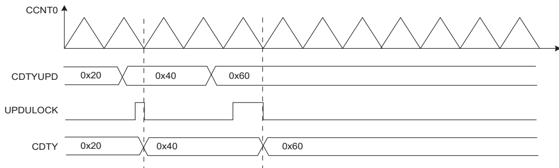
Figure 51-19. Method 1 (UPDM = 0)
