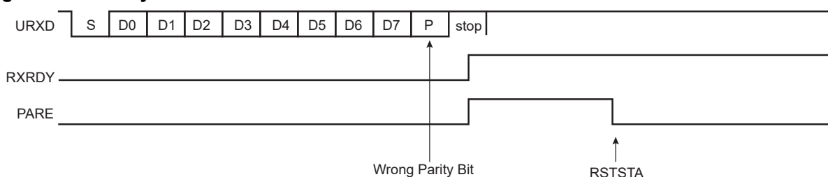
Figure 47-7. Parity Error
