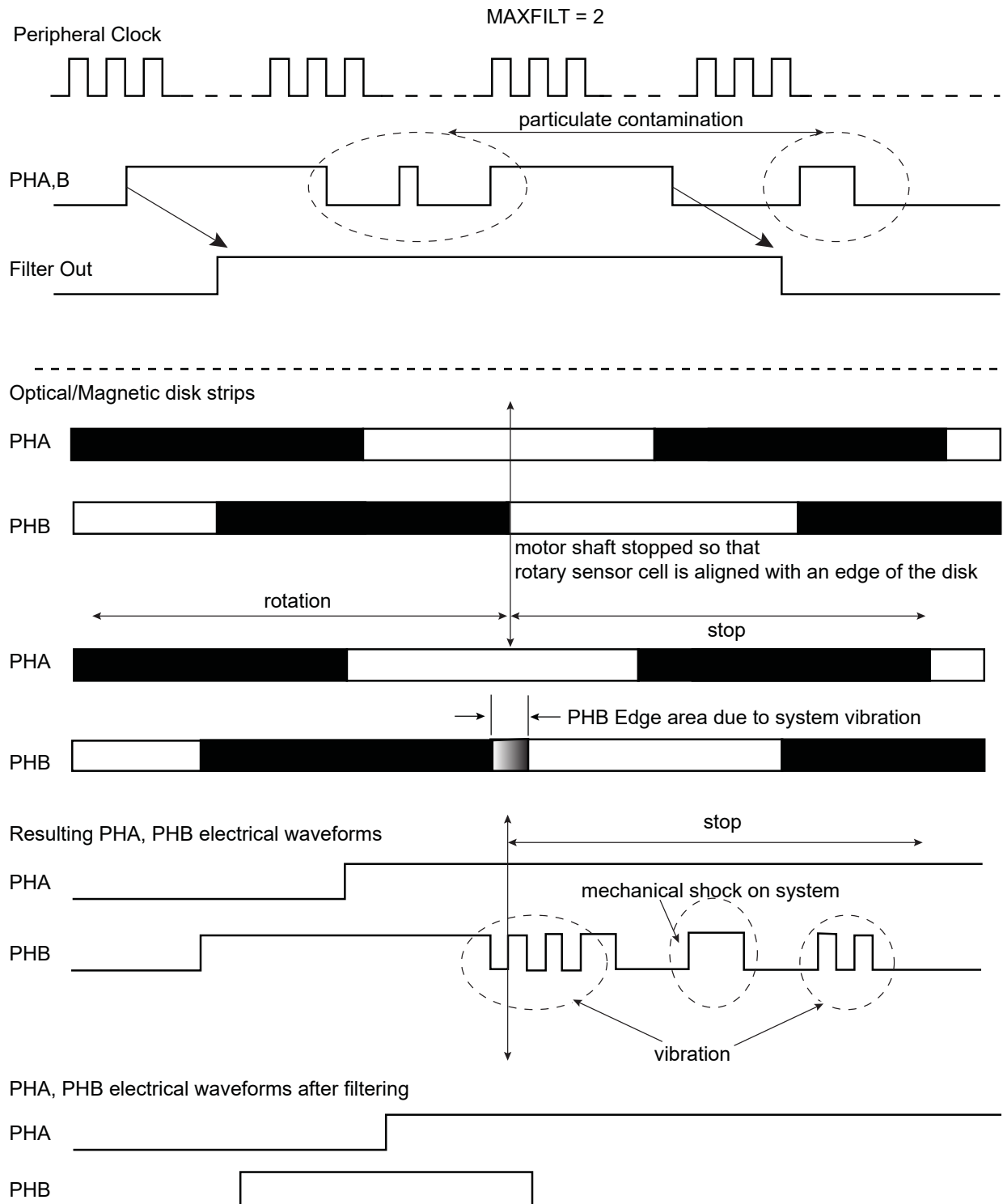
Figure 50-19. Filtering Examples
