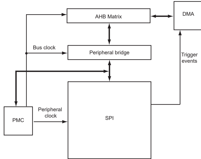
Figure 41-1. Block Diagram
