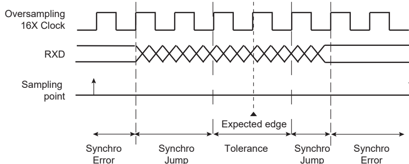
Figure 46-10. Bit Resynchronization
