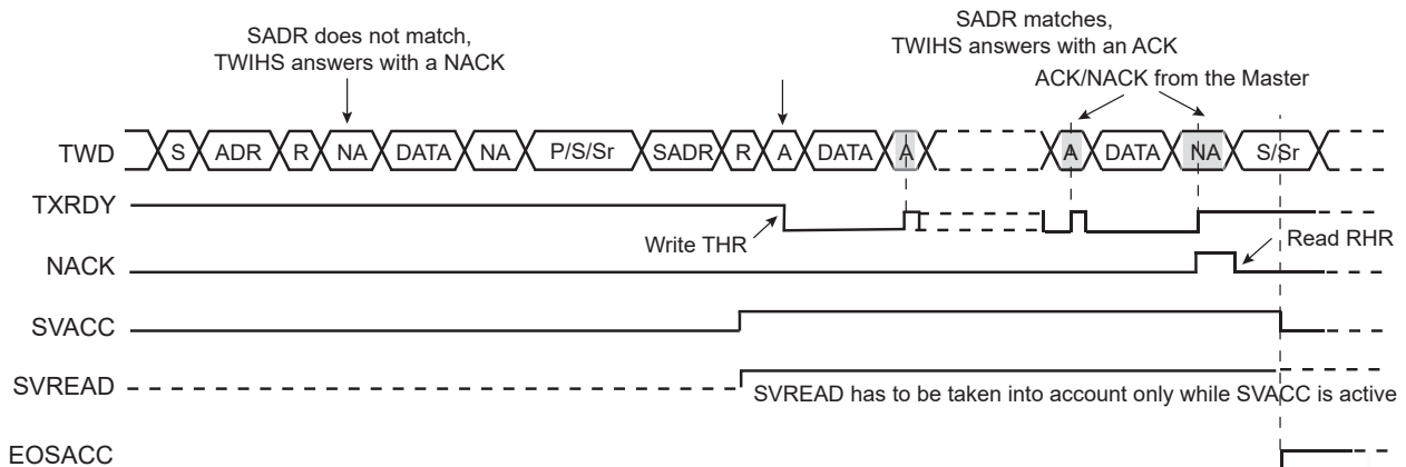
Figure 43-31. Read Access Ordered by a Master
