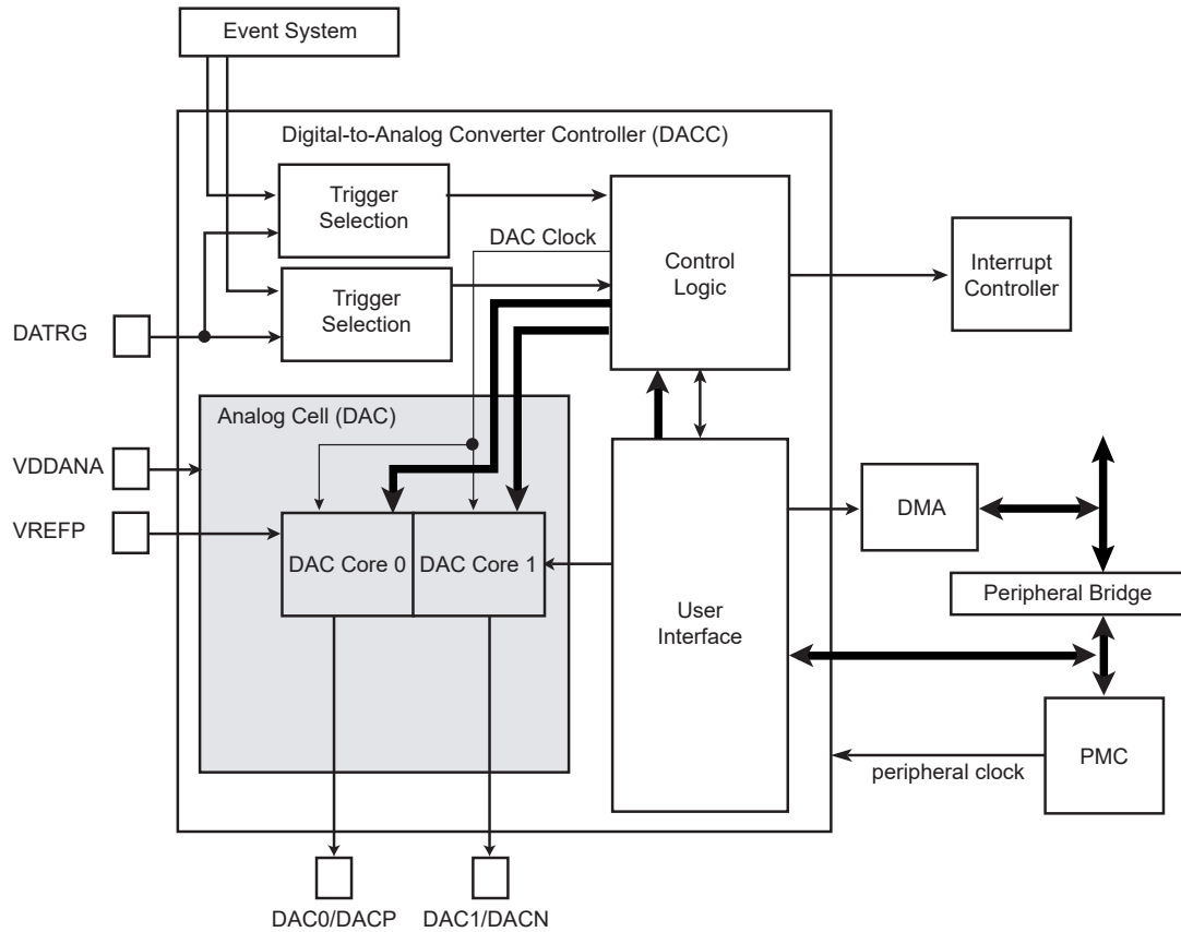
Figure 53-1. Block Diagram
