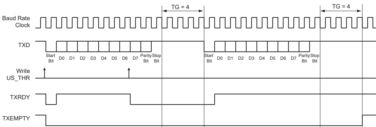
Figure 46-22. Timeguard Operations
