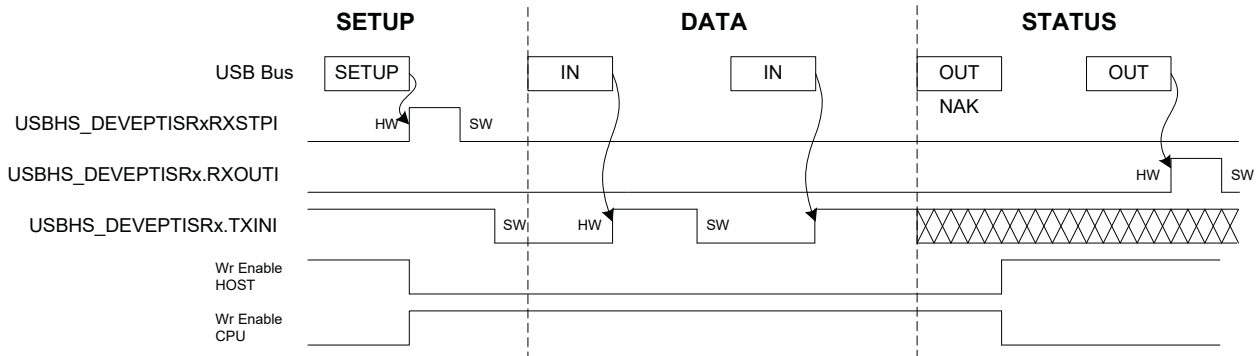
Figure 39-10. Control Read
