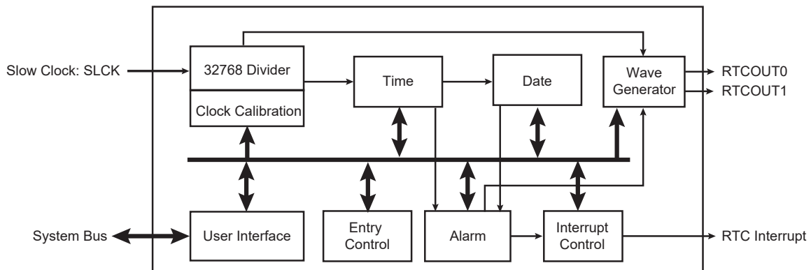
Figure 27-1. Real-time Clock Block Diagram
