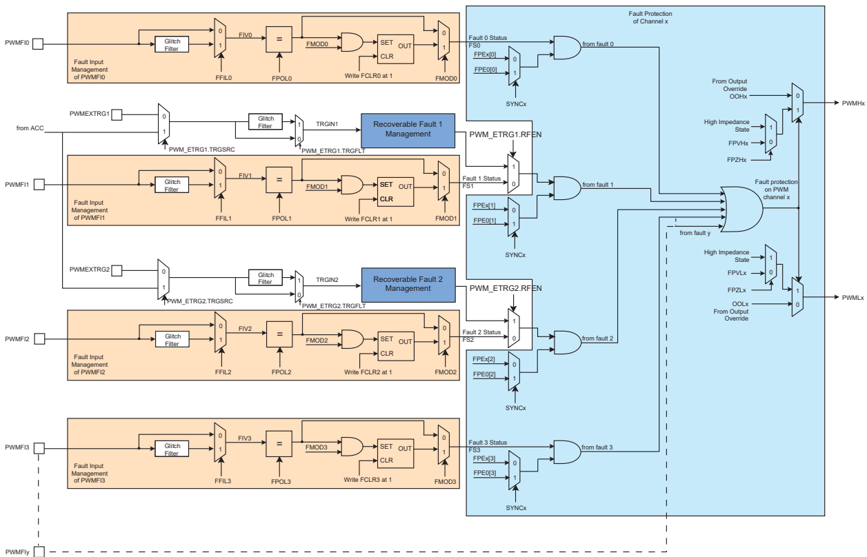
Figure 51-16. Fault Protection
