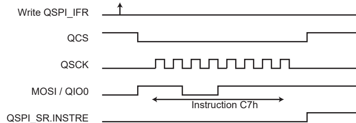
Figure 42-11. Instruction Transmission Waveform 1
