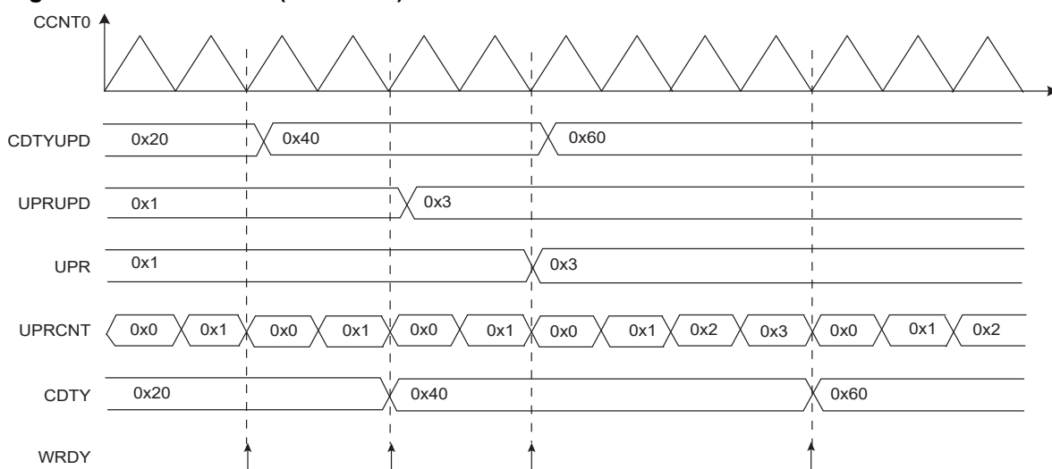
Figure 51-20. Method 2 (UPDM = 1)
