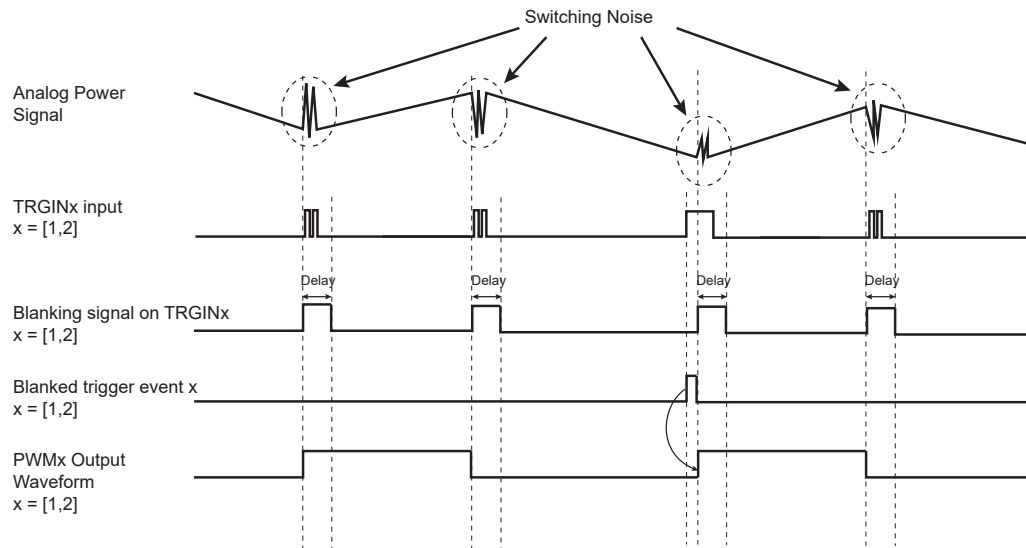
Figure 51-33. Leading-Edge Blanking
