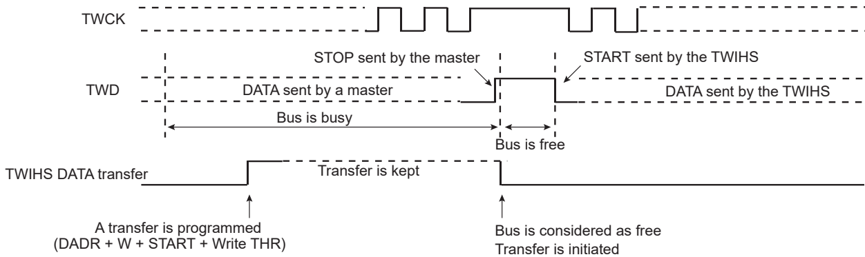
Figure 43-29. Arbitration Cases
