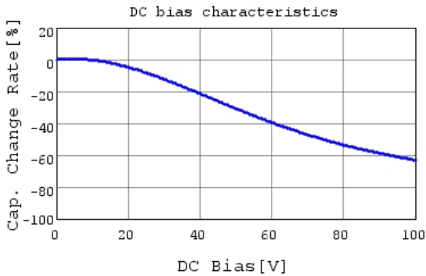
RHEL82A153K0DBH03A C-DC bias capchange, 25.0
