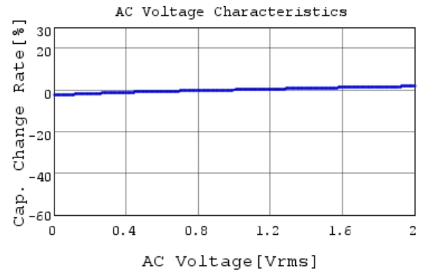
RHEL82A153K0DBH03A C-AC Voltage capchange, 1
