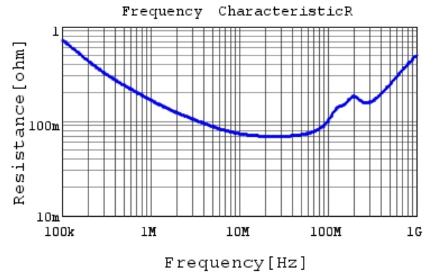
RHEL82A153K0DBH03A R DCOV, 25degC
