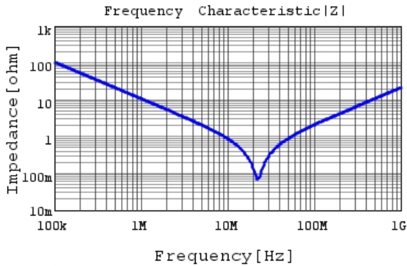
RHEL82A153K0DBH03A |Z| DCOV, 25degC
