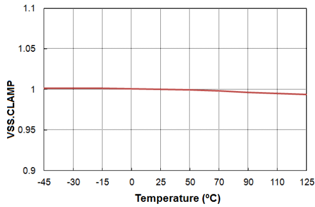
Figure 11. V SS,CLMP vs. Temperature
