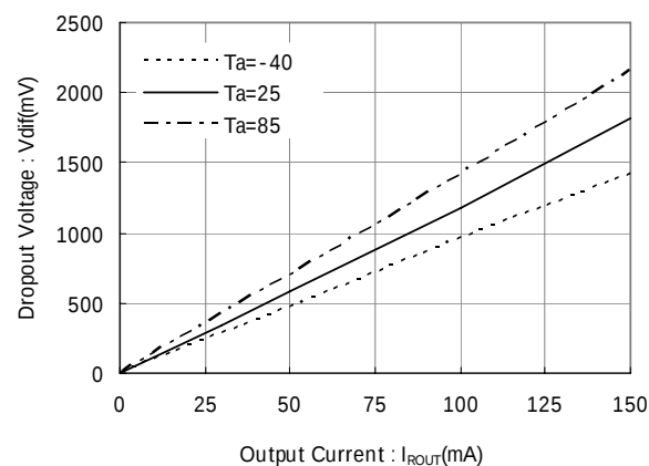
XC6408D/E ( V_{ROUT}=5.0V )
