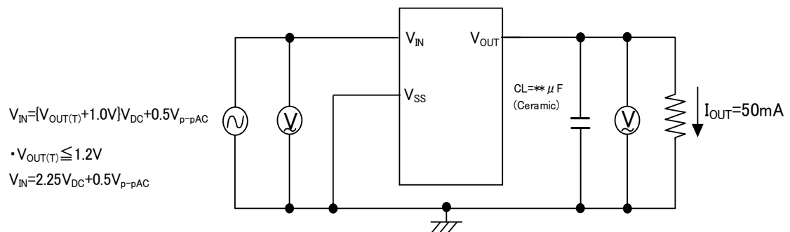
Circuit ③
