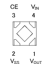
USPQ-4B04 (BOTTOM VIEW)
