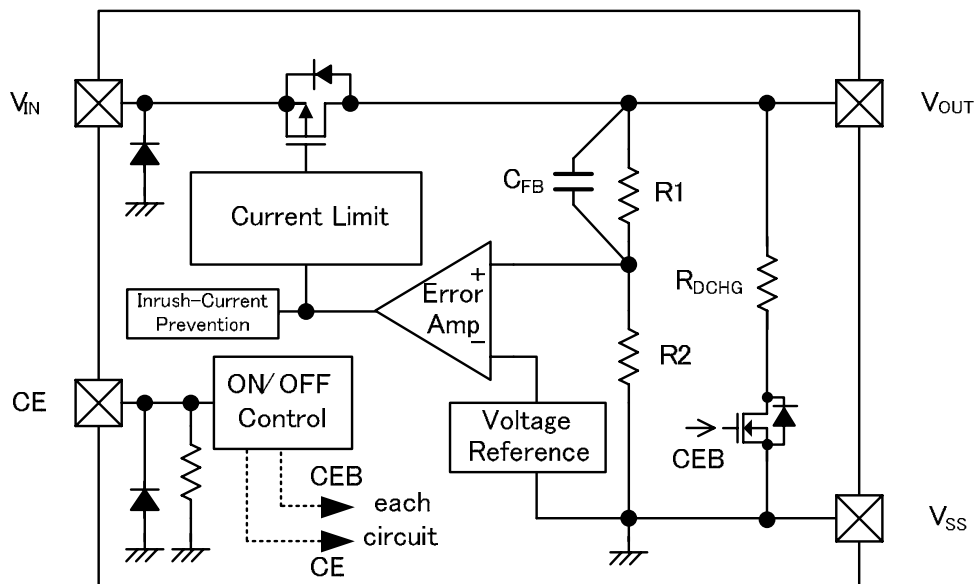
XC6233 Series, Type H
