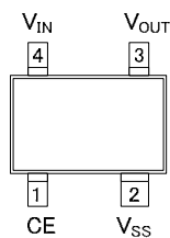
SSOT-24 (TOP VIEW)
