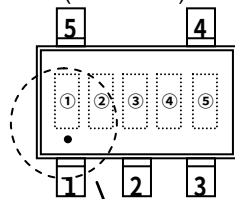
SOT-25 (Under-dot)
