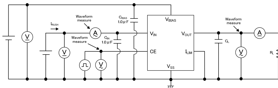
CIRCUIT⑤
