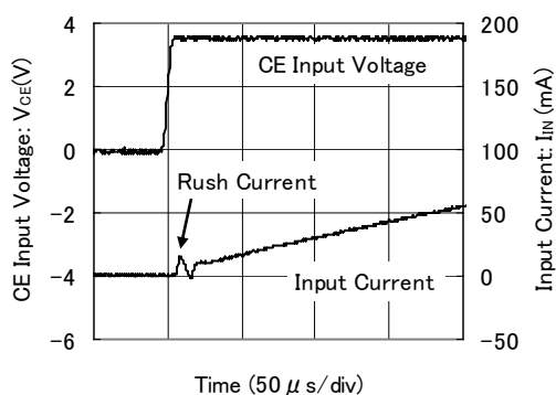
XC6604A121xR-G
