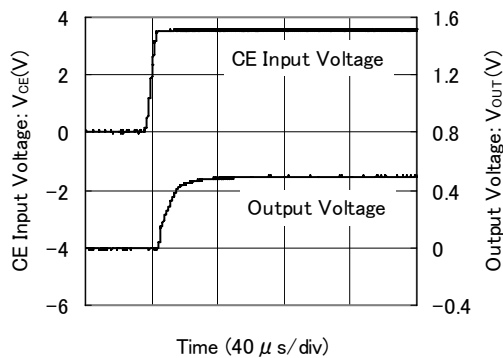
XC6604B121xR-G
