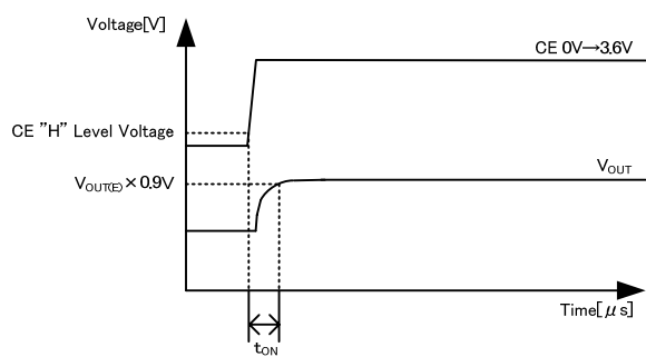
XC6604 Series, Type B
