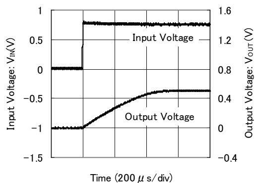
XC6604A121xR-G
