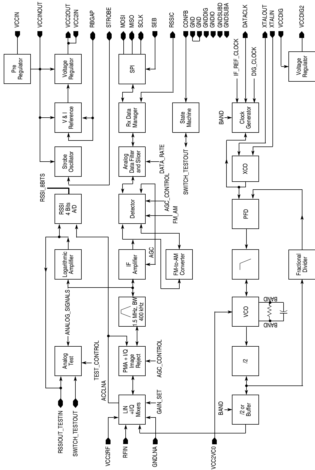
Figure 1. Block Diagram
