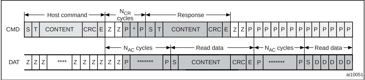
Figure 24. Multiple Block Read command
