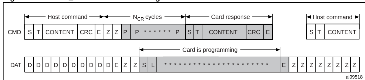
Figure 28. STOP_TRANSMISSION during data transfer from the host
