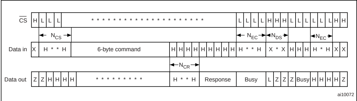
Figure 39. Host command to card response - card is busy
