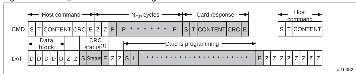
Figure 29. STOP_TRANSMISSION during CRC status transfer from card
