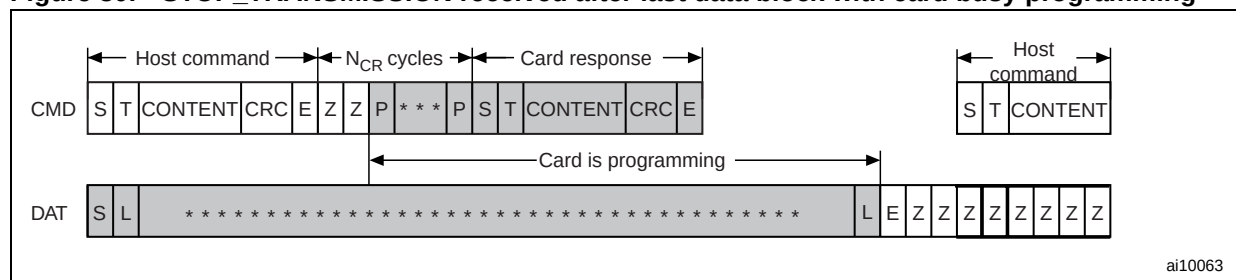
Figure 30. STOP_TRANSMISSION received after last data block with card busy programming
