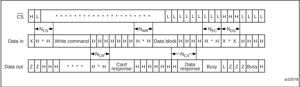
Figure 45. Single block write operation
