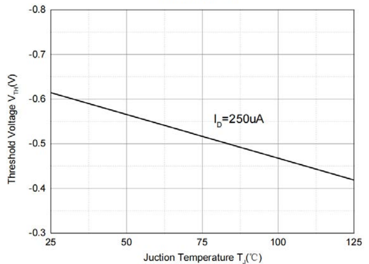
Threshold Voltage
