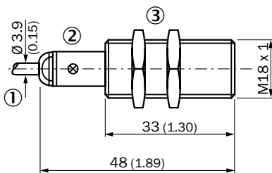
IME18 Short-body housing, cable, flush
