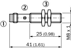
IME08 Short-body housing, connector, flush
