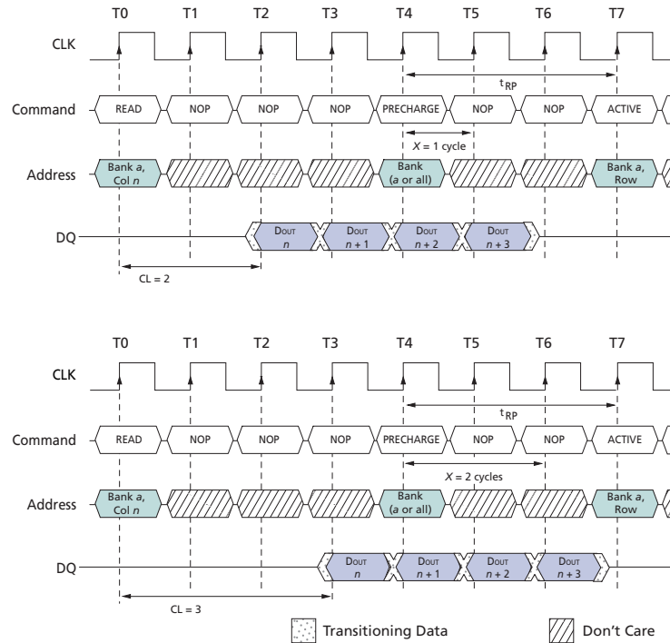
Figure 14: READ-to-PRECHARGE
