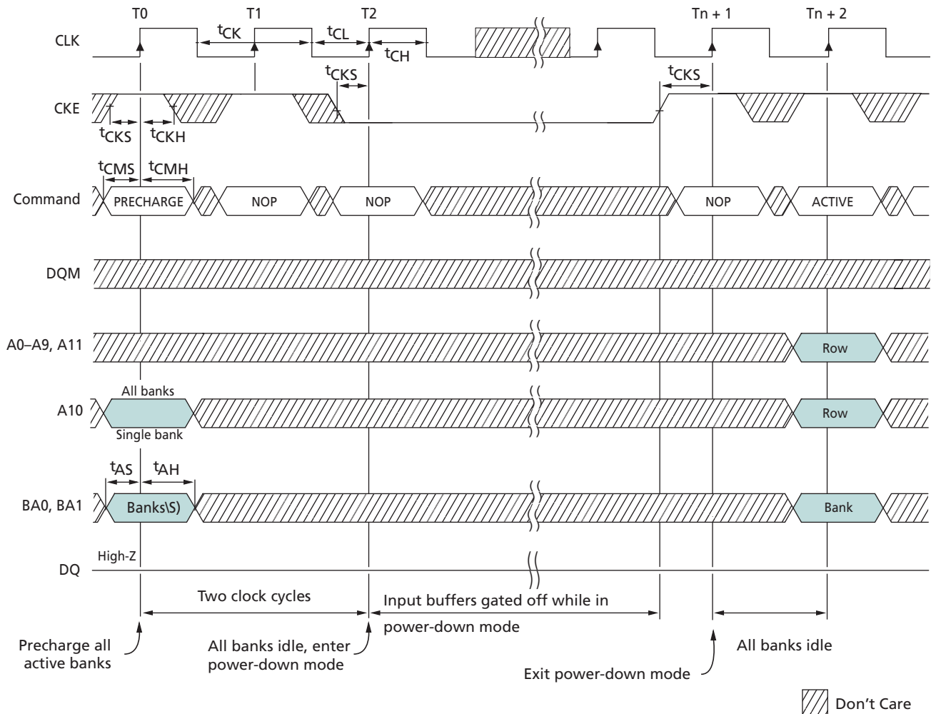
Figure 33: Power-Down Mode
