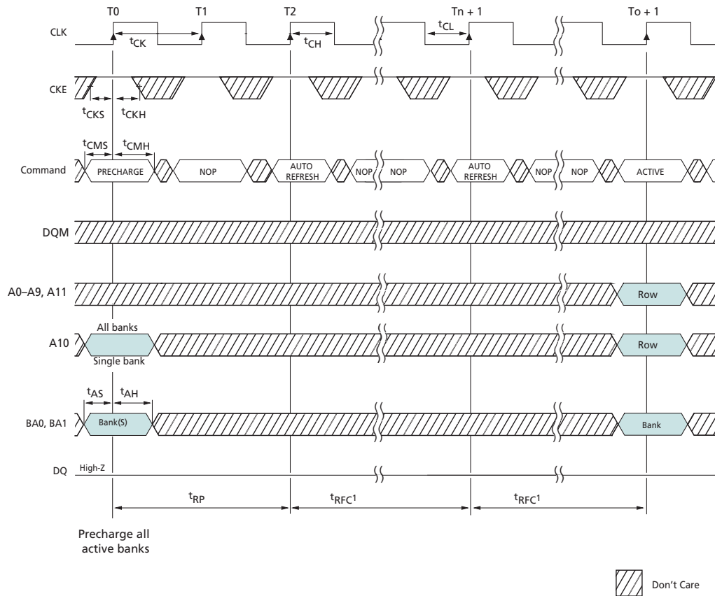
Figure 35: Auto Refresh Mode
