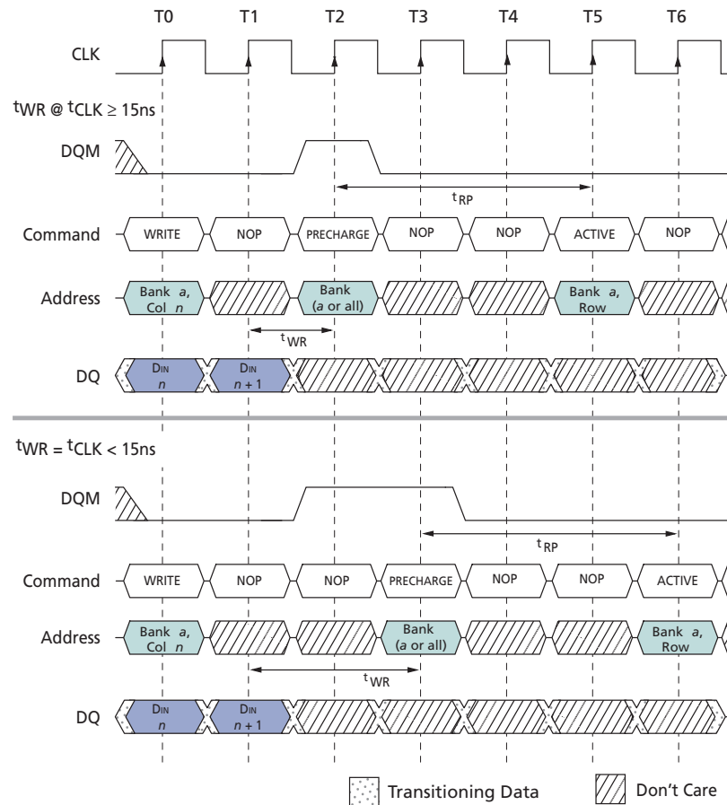
Figure 21: WRITE-to-PRECHARGE
