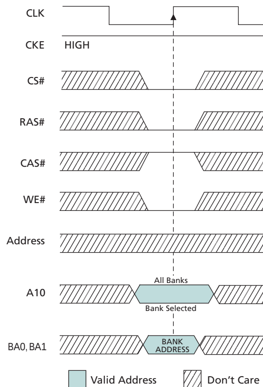
Figure 23: PRECHARGE Command
