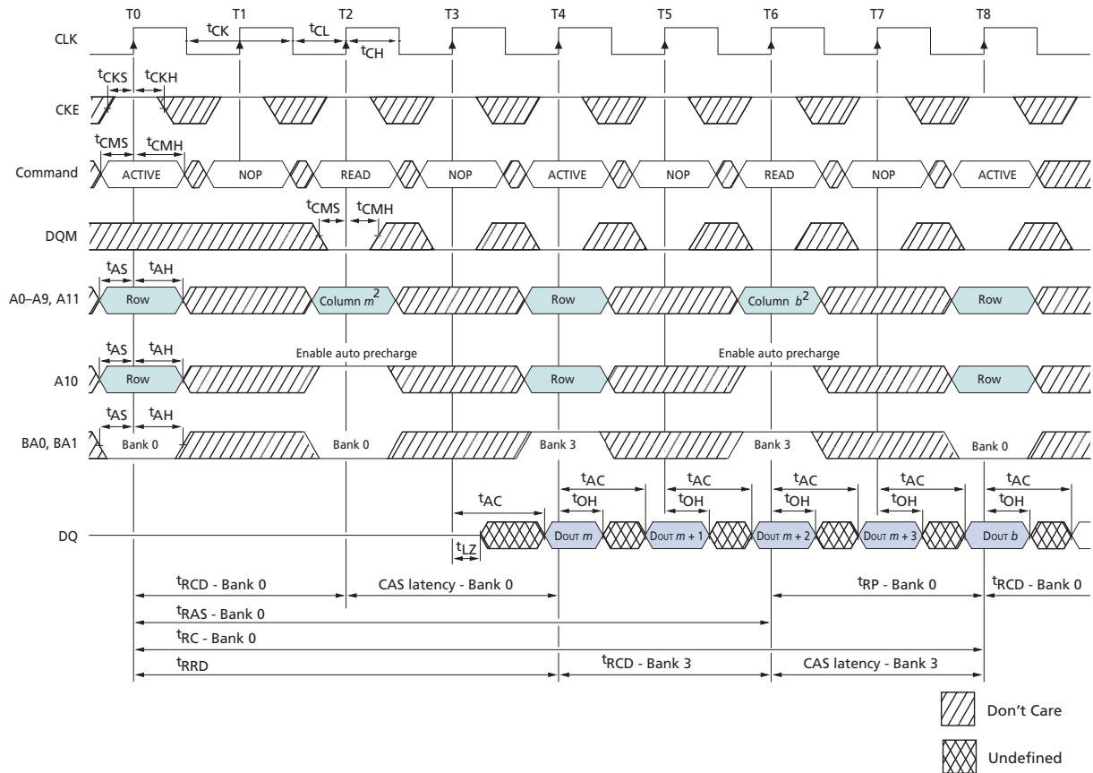
Figure 41: Alternating Bank Read Accesses
