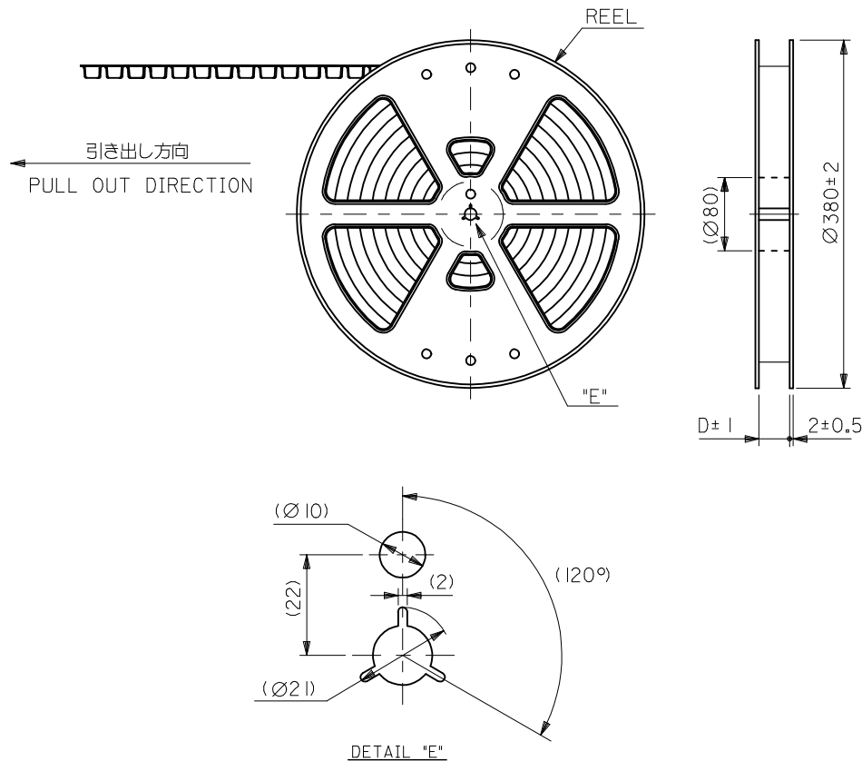
DETAIL "E"
