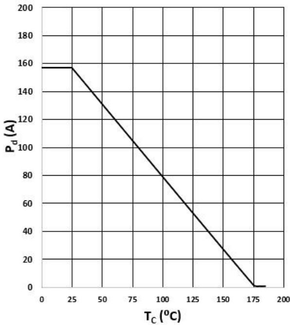
Figure 3: Power Dissipation
