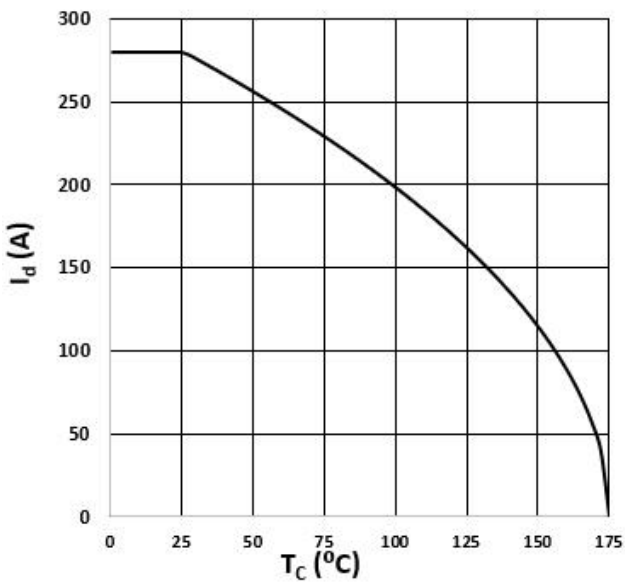
Figure5: Drain Current
