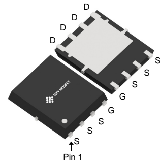
DFN5X6-8L (TDSON-8)
