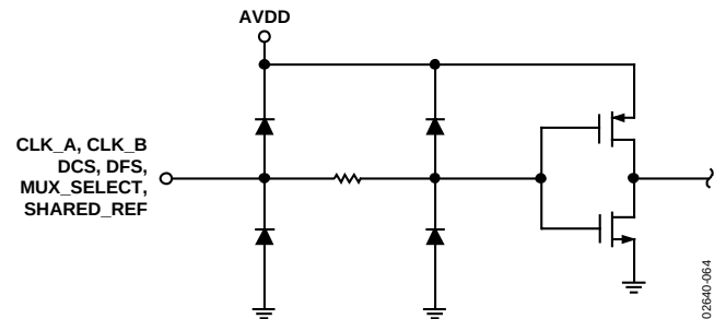
Figure 30. Equivalent Digital Input Circuit
