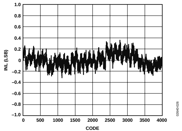
Figure 26. AD9238-65 Typical INL
