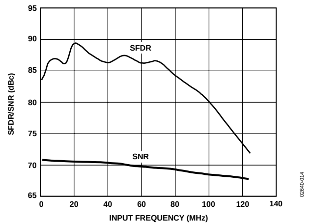
Figure 14. AD9238-40 Single-Tone SNR/SFDR vs. f_{IN}
