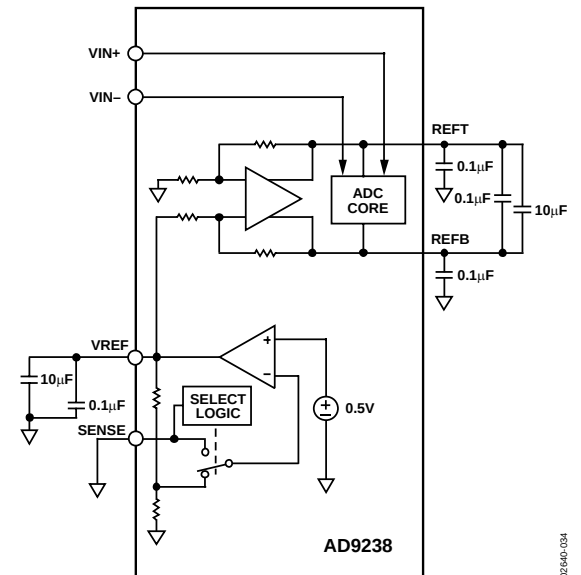
Figure 34. Internal Reference Configuration
