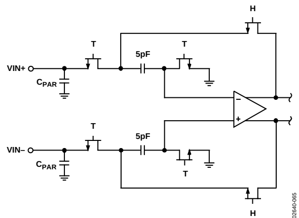
Figure 31. Switched-Capacitor Input
