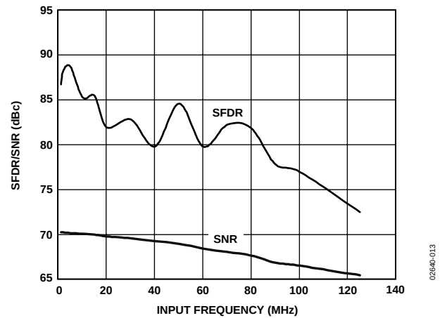
Figure 13. AD9238-65 Single-Tone SNR/SFDR vs. f_{IN}
