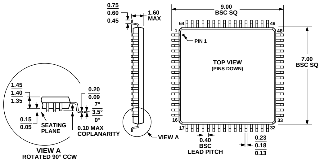
Figure 59. 64-Lead Low Profile Quad Flat Package [LQFP]
