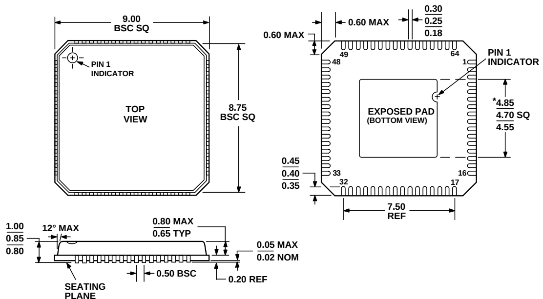
Figure 60. 64-Lead Lead Frame Chip Scale Package [LF CSP_VQ]
