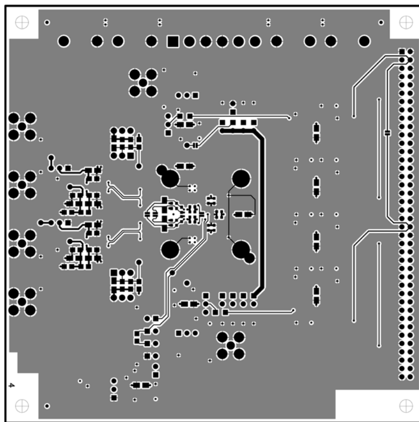
Figure 47. PCB Bottom Layer
