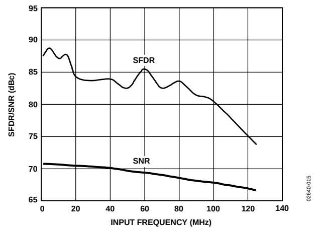
Figure 15. AD9238-20 Single-Tone SNR/SFDR vs. f_{IN}
