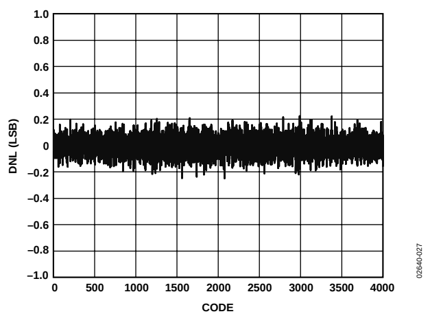
Figure 27. AD9238-65 Typical DNL
