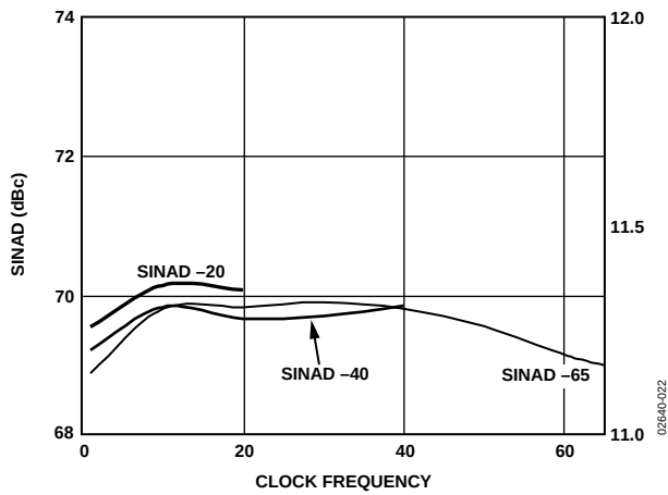
Figure 22. SINAD vs. FS with Nyquist Input
