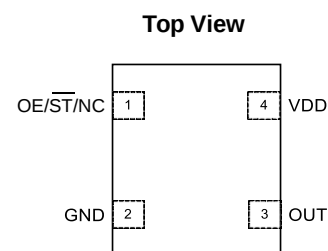
Figure 1. Pin Assignments
