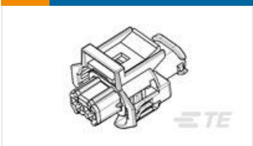
TE Part #936059-1 2.8MM SLD 2P PLUG ASSY
