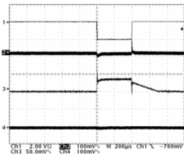
Channel 1: Current Sunk into of VTT, 2.0 A/div Channel 2: VDDQ Output Voltage, AC-Coupled, 100 mV/div Channel 3: VTT Output Voltage, AC-Coupled, 50 mV/div Channel 4: V1P5 Output Voltage, AC-Coupled, 100 mV/div Time Base: 200 μs/div
