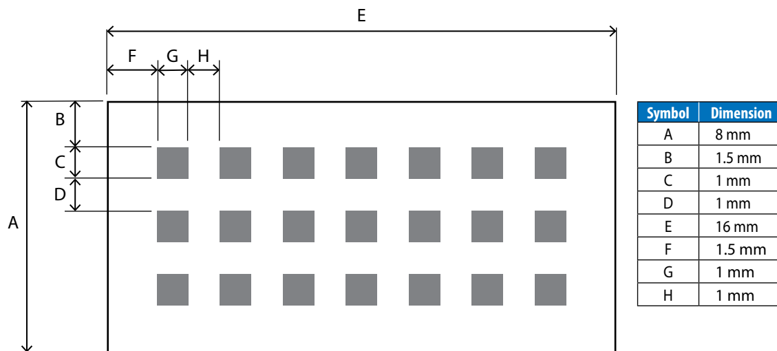
Figure 9: Footprint mechanical outline and pin numbering. (Top view)
