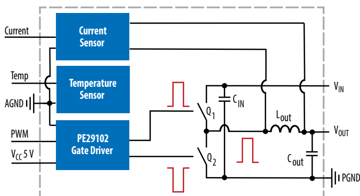
Figure 1. Block Diagram of EPC9204 Development Board.
