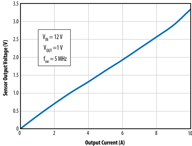
Figure 5: Typical Current Sensor Output Curve for EPC9204 Development Board with V_{IN} = 12\text{ V} to 1\text{ V}_{OUT} , 5\text{ MHz}
