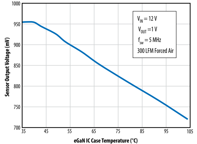
Figure 6: Example Temperature Sensor Output Curve for EPC9204 Development Board with V_{IN} = 12\text{ V} to 1\text{ V}_{OUT} , 5\text{ MHz} , 300 LFM Forced Air Cooling
