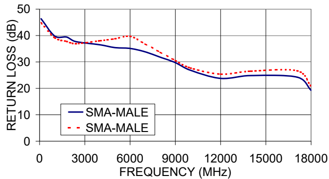
086-36SM+ RETURN LOSS
