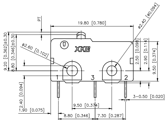
Left Angled PCB Terminals
