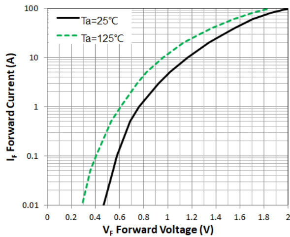
Figure 1. Forward Characteristic(typ.)
