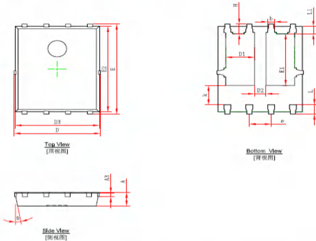
PDFNWB5×6-8L-A PACKAGE OUTLINE DIMENSIONS
