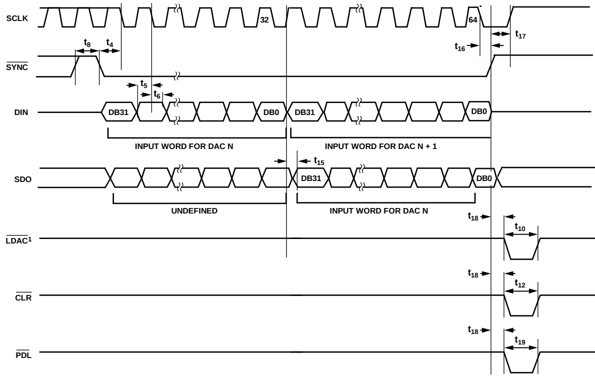
Figure 4. Daisy-Chain Timing Diagram
