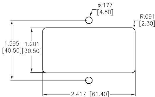
RECOMMENDED PANEL CUT
