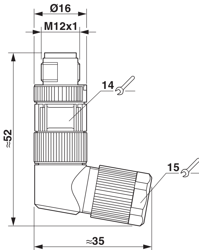
Dimensional drawing
