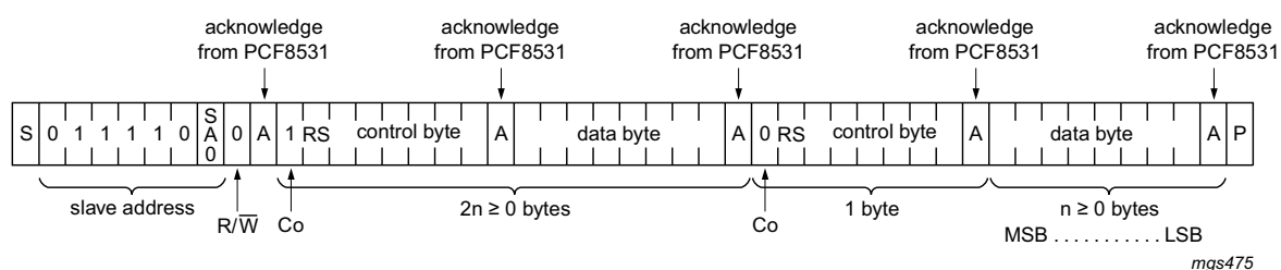
Fig 19. Master transmits to slave receiver; write mode
