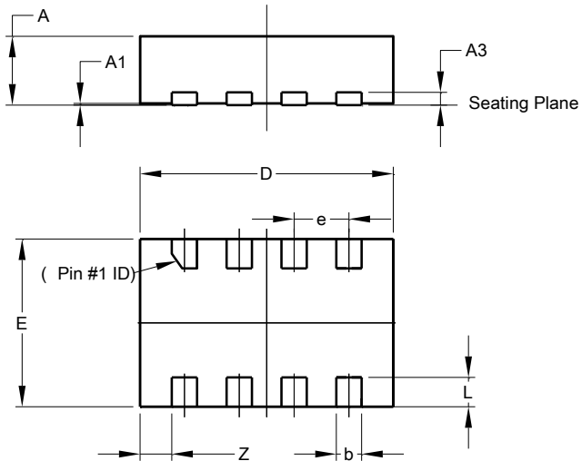
V-DFN3020-8
