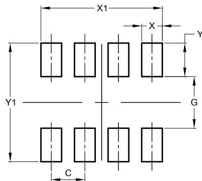
V-DFN3020-8
