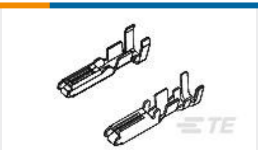
TE Part #345206-1 070 SERIES RECEPT.
