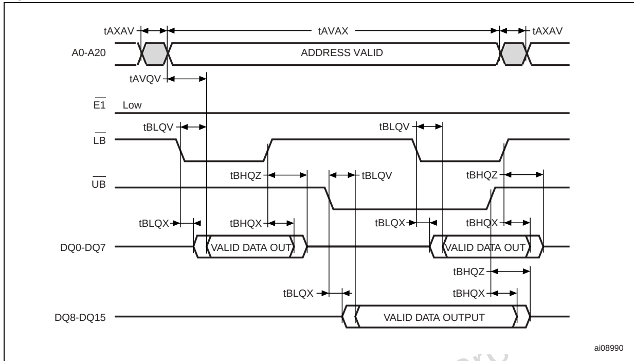
Figure 9. \overline{\text{UB}}/\overline{\text{LB}} Controlled, Read Mode AC Waveforms
