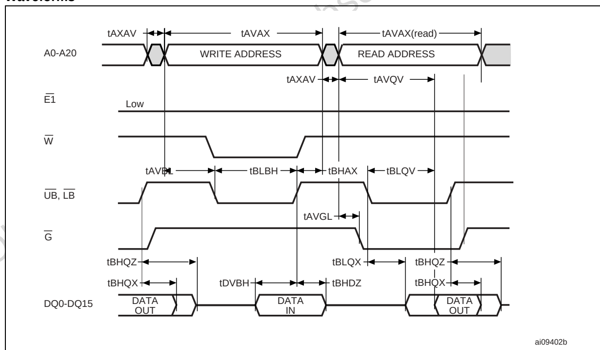
Figure 21. Output Enable, Write Enable and \overline{\text{UB/LB}} Controlled, Read and Write Mode AC Waveforms
