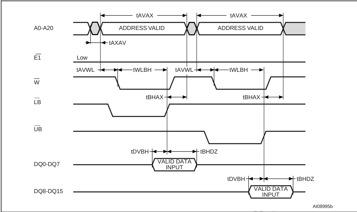
Figure 14. Write Enable and \overline{\text{UB}}/\overline{\text{LB}} Controlled, Write AC Waveforms 1
