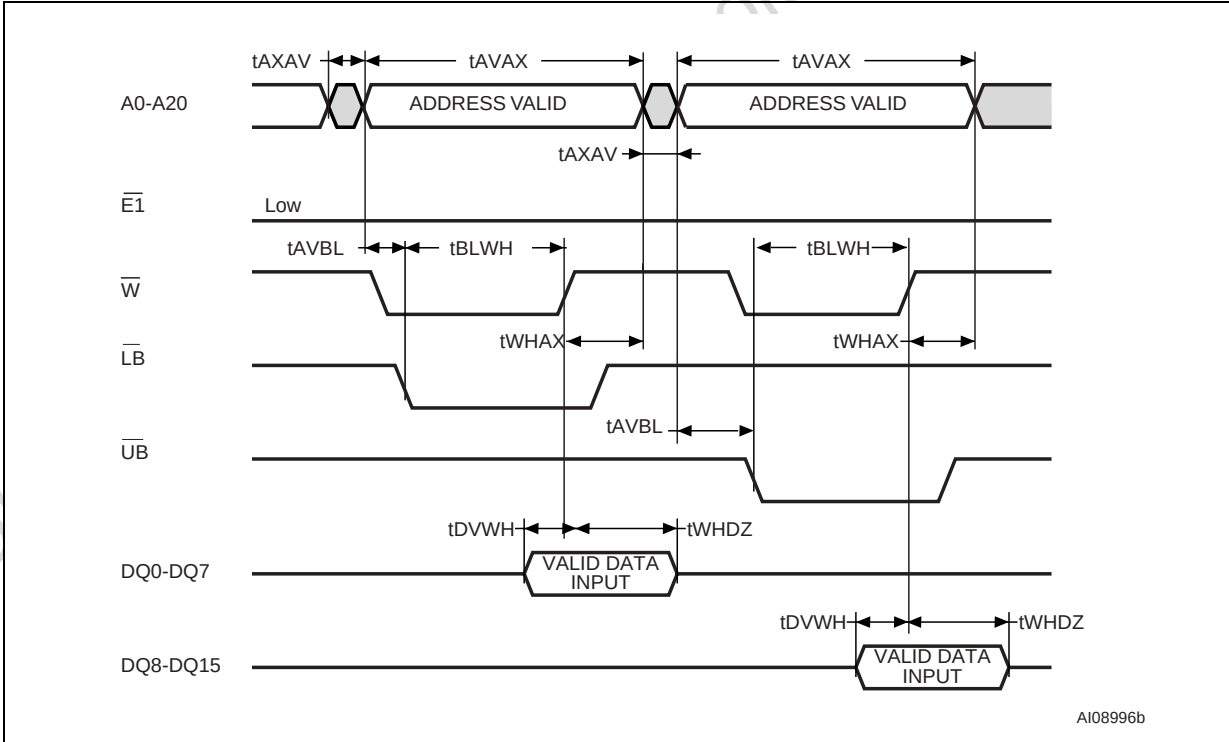
Figure 15. Write Enable and \overline{\text{UB}}/\overline{\text{LB}} Controlled, Write AC Waveforms 2
