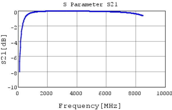
GRM0335C2A6R9WA01 S21 DCOV, 25degC
