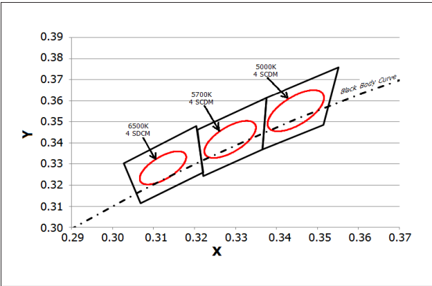
Figure 19: Cool White Test Bins in xy Color Space
