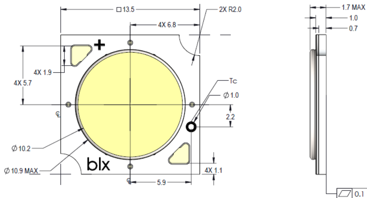
Figure 17: Drawing for V10 LED Array
