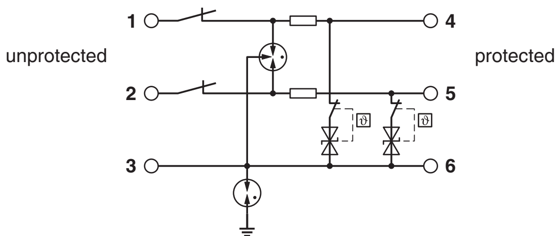
Circuit diagram
