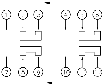
SCHEMATIC
