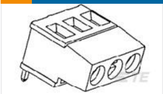
TE Part #1-1546073-2 12POS 5.08MM TERMINAL BLOCK
