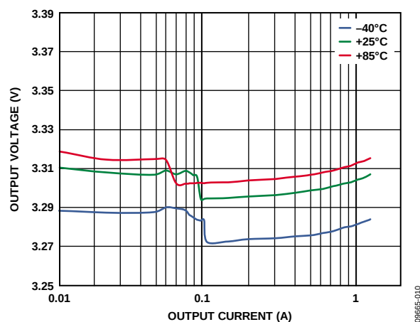
Figure 10. Buck Load Regulation Across Temperature, V_{OUT1} = 3.3 V, Auto Mode
