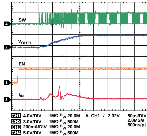
Figure 6. Buck Startup, V OUT1 = 3.3 V, I OUT = 20 mA
