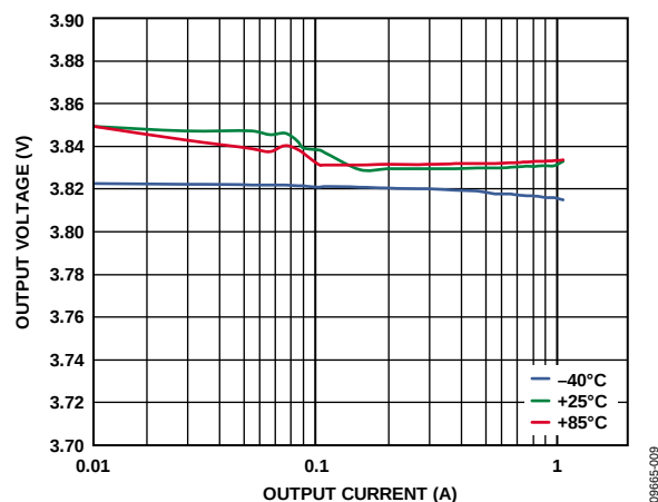
Figure 9. Buck Load Regulation Across Temperature, V_{OUT1} = 3.8 V, Auto Mode
