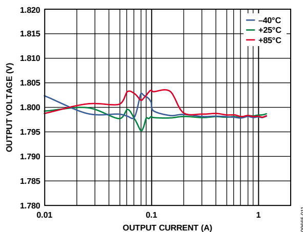
Figure 11. Buck Load Regulation Across Temperature, V_{OUT1} = 1.8 V, Auto Mode
