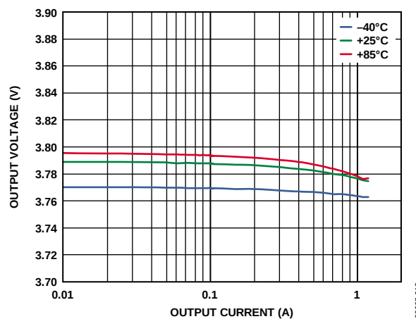
Figure 13. Buck Load Regulation Across Temperature, V_{OUT1} = 3.8 V, PWM Mode
