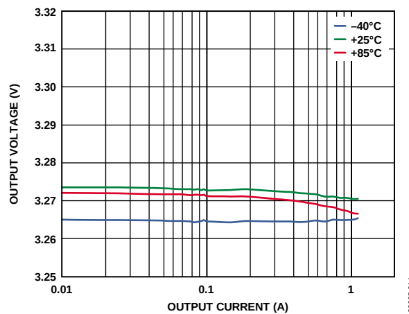
Figure 14. Buck Load Regulation Across Temperature, V_{OUT1} = 3.3 V, PWM Mode
