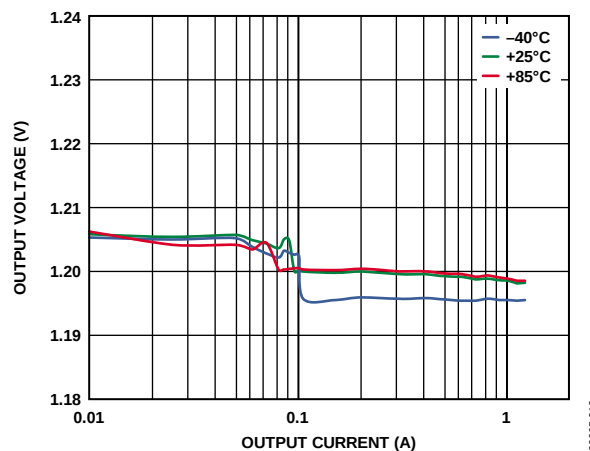
Figure 12. Buck Load Regulation Across Temperature, V_{OUT1} = 1.2 V, Auto Mode
