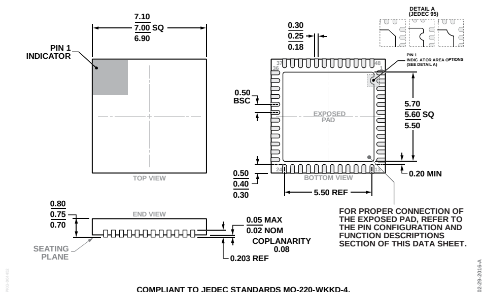
Figure 65. 48-Lead Lead Frame Chip Scale Package [LFCSP] 7 mm × 7 mm Body and 0.75 mm Package Height (CP-48-13)
