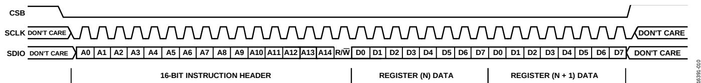
Figure 57. Serial Control Port Write—LSB First, Address Increment, Two Bytes of Data
