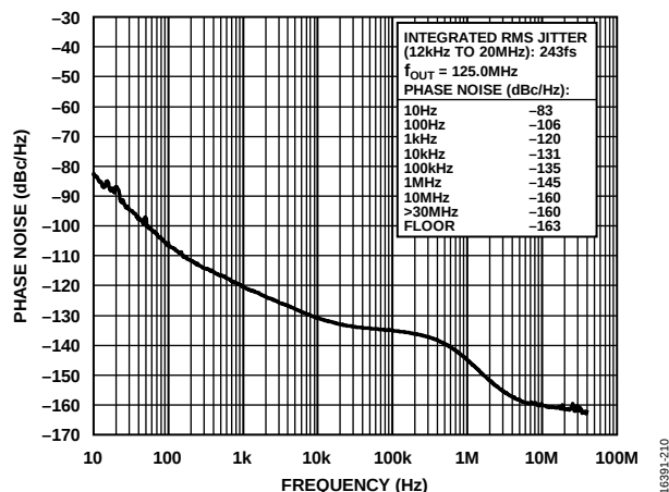
Figure 12. Absolute Phase Noise (PLL1, Configuration 4, HCSL Mode, f_{REF} = 125\text{ MHz} , f_{OUT} = 125\text{ MHz} , f_{COMP} = 19.2\text{ MHz} TCXO, f_{SYS} = 52\text{ MHz} Crystal, BW_{DPLL} = 0.1\text{ Hz} , Phase Buildout Mode)
