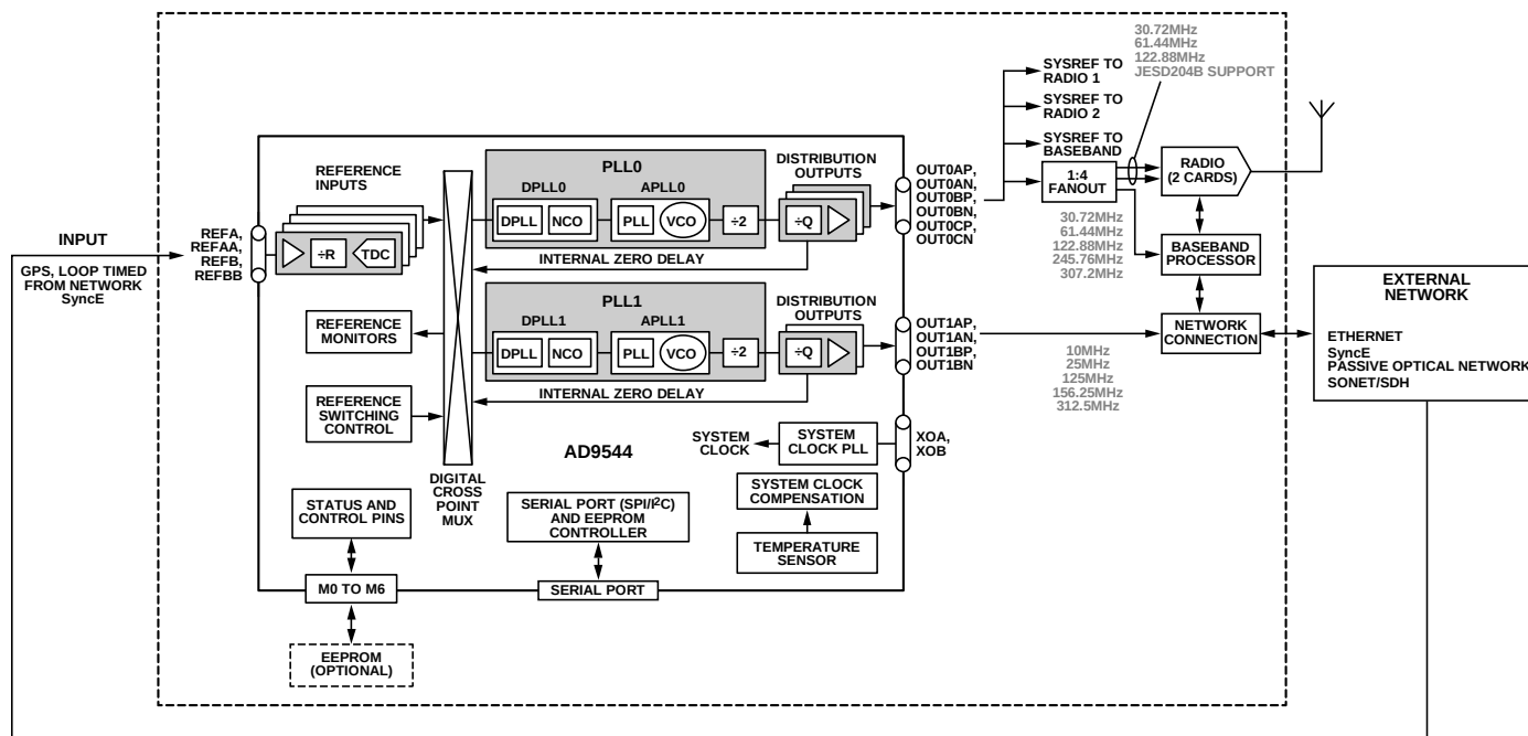
Figure 42. Small Cell Application
