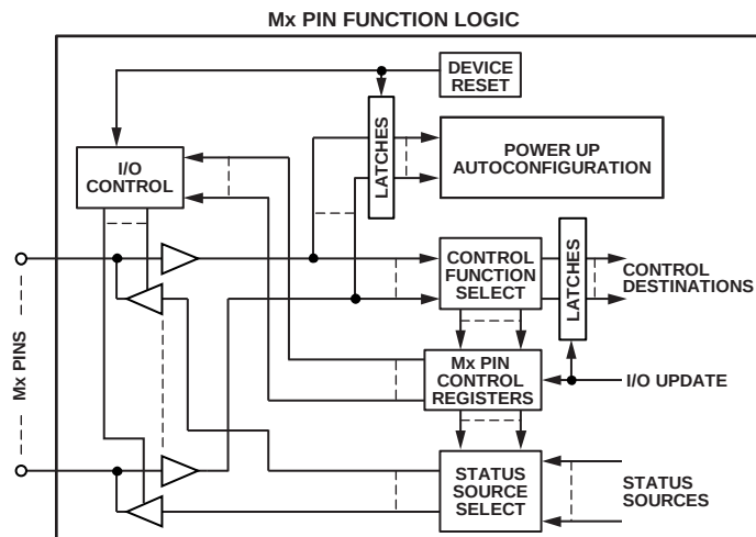
Figure 46. Mx Pin Logic
