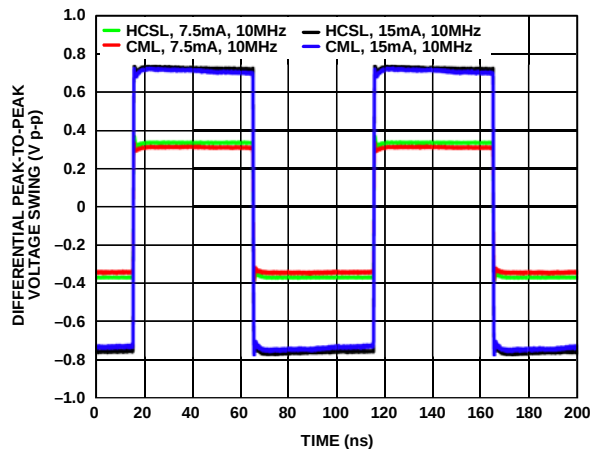
Figure 17. 10 MHz Output Waveforms for Various Driver Settings; HCSL Drivers Terminated 50\ \Omega to GND per Figure 32; CML Drivers Terminated 50\ \Omega to 1.8 V per Figure 33
