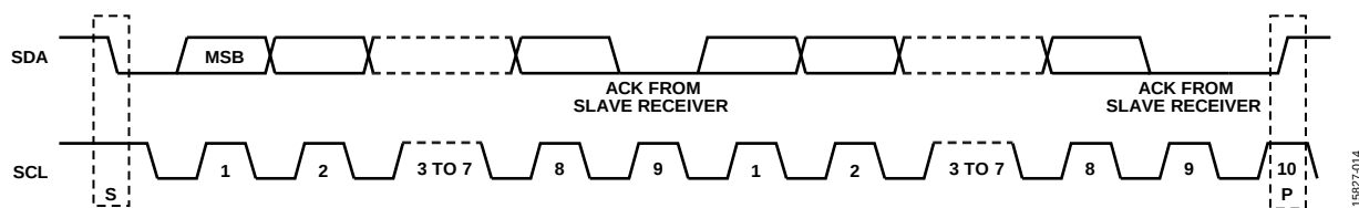
Figure 62. Acknowledge Bit
