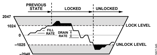
Figure 50. Lock Detector Diagram
