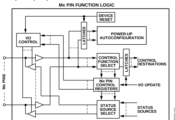
Figure 47. Mx Pin Function Logic
