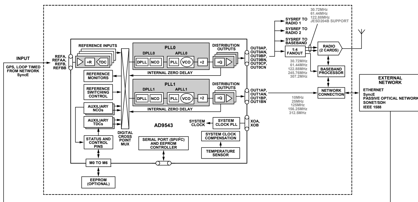
Figure 42. AD9543 Small Cell Application
