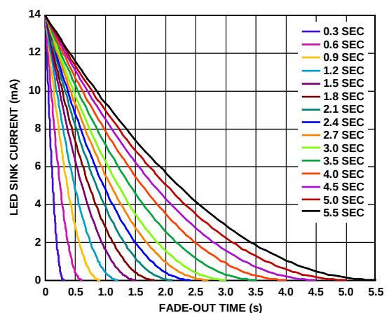
Figure 45. Square Law Fade-Out Times
