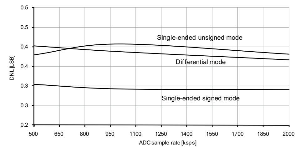
Figure 37-39. DNL error vs. sample rate. T = 25°C, V CC = 2.7V, V REF = 1.0V external.
