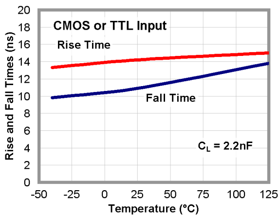
Figure 38. Rise and Fall Times vs. Temperature
