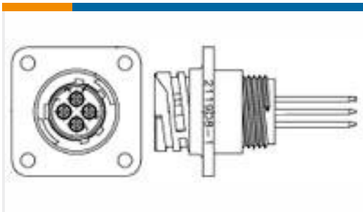
TE Part #1-788130-1 CPC RCPT,PSTD,SZ 11-4 LF
