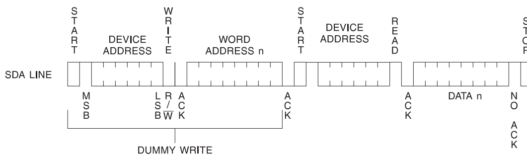
Figure 11. Random Read
