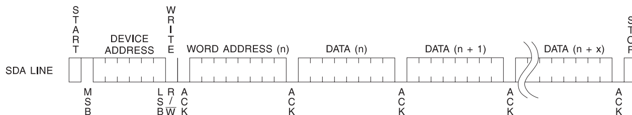
Figure 9. Page Write
