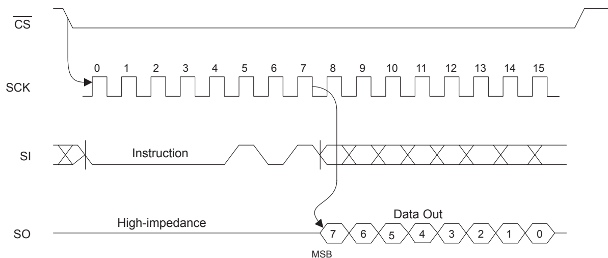
Figure 7-4. RDSR Timing
