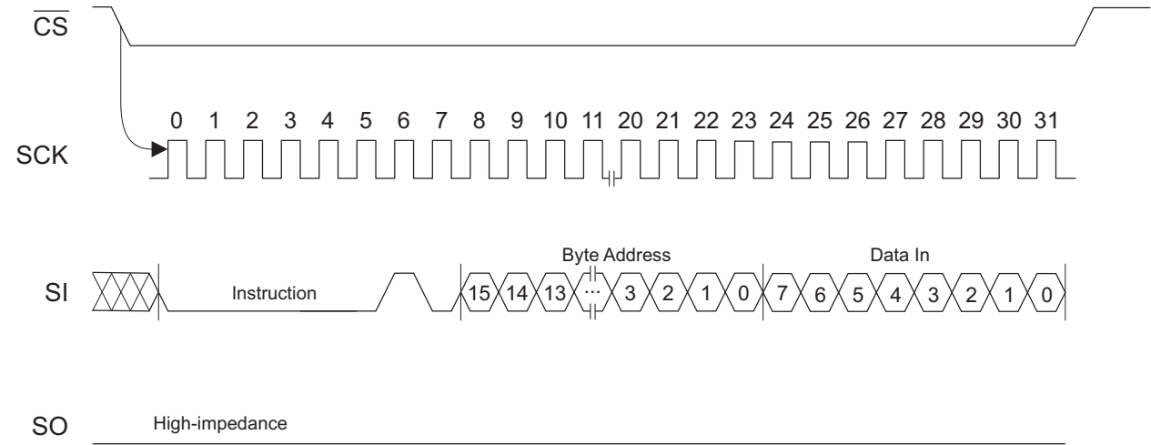
Figure 7-7. Write Timing
