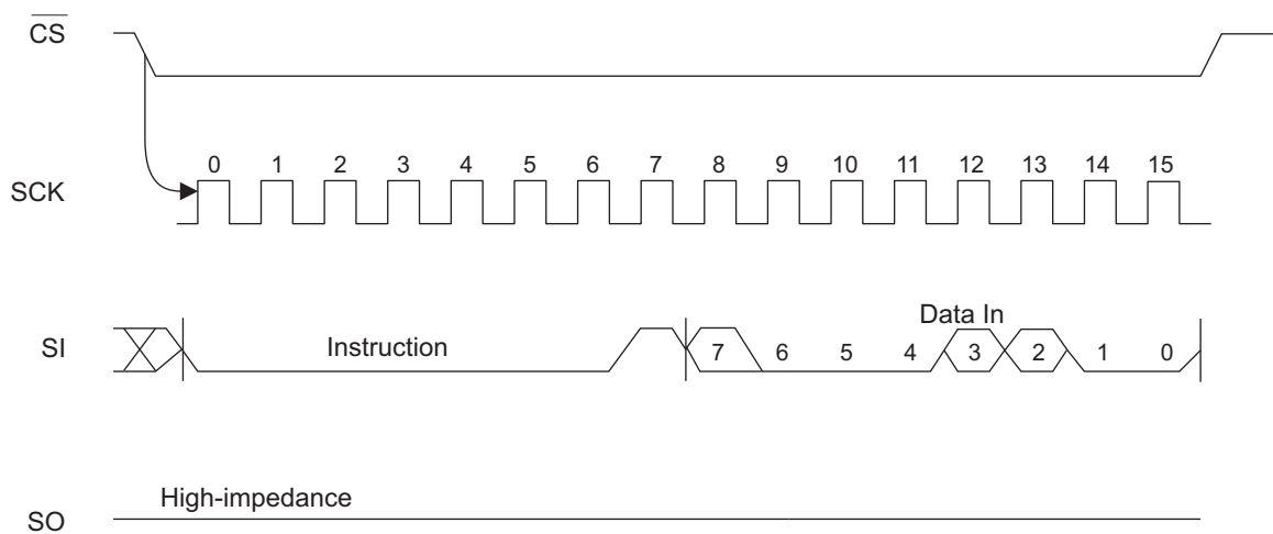
Figure 7-5. WRSR Timing
