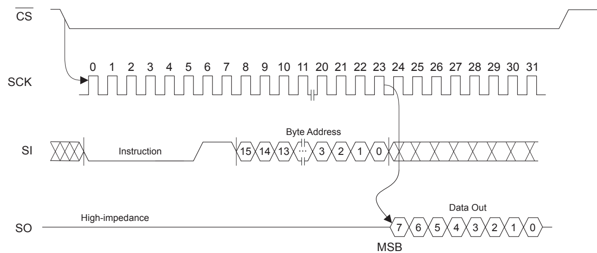
Figure 7-6. Read Timing
