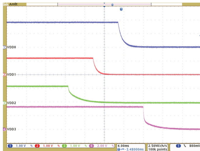
Detailed Supplies shutdown SEQUENCE B
