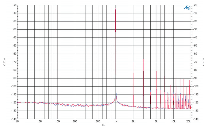
DAC playback ( Path 1) - Load 32 Ohms AC coupled 20mW Ouput Power - F_s = 48\text{kHz} - 32kpts FFT
