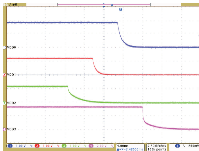
Detailed Supplies Start-Up SEQUENCE B
