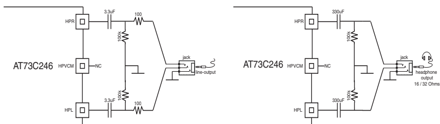
Figure 12-31. AC Coupled Output Application Circuits
