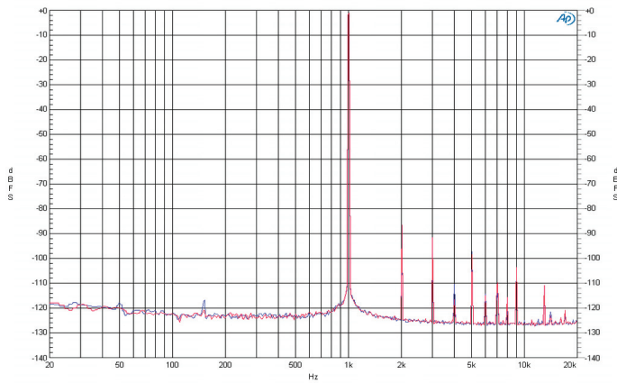
Line Record (path 7) -1 dBV / 1kHz Input - F_s = 48\text{kHz} - 32kpts FFT
