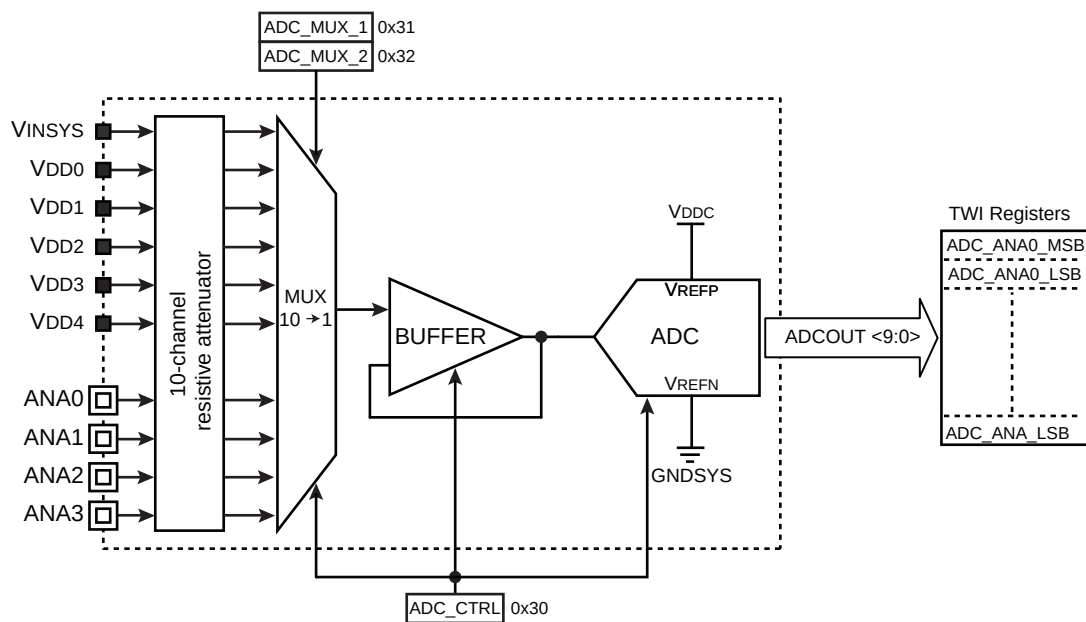
Figure 11-9. Measurement Bridge and 10-bit ADC Block Diagram.
