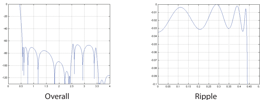
Figure 12-11. DAC Type 0 Frequency Response
