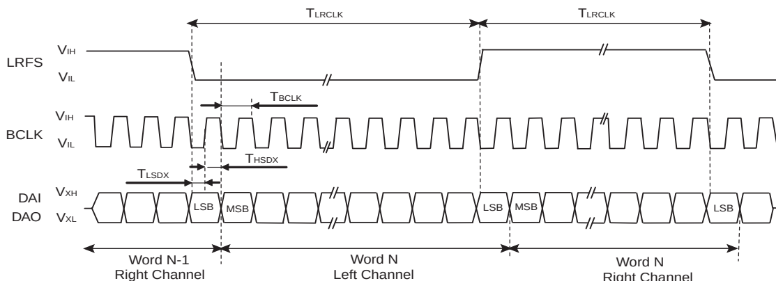
Figure 12-10. Timing Diagram of data interface (I 2 S Mode)
