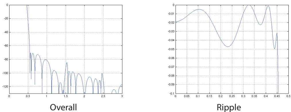
Figure 12-13. DAC Type 2 Frequency Response
