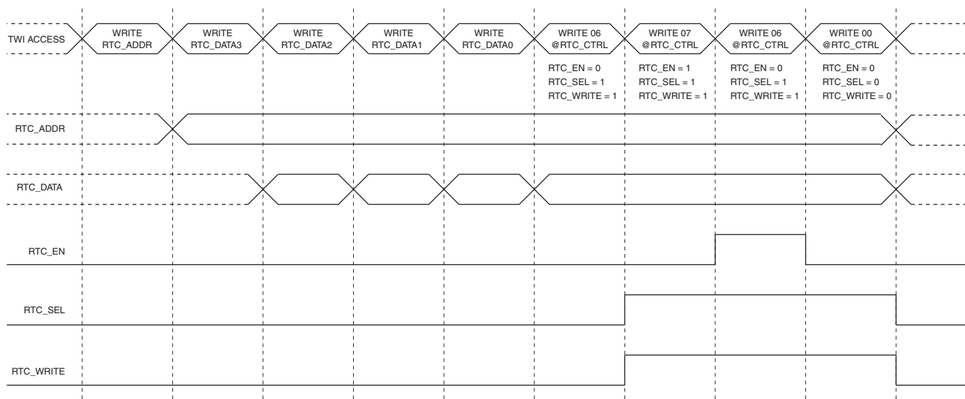
Figure 11-12. RTC Write Operation
