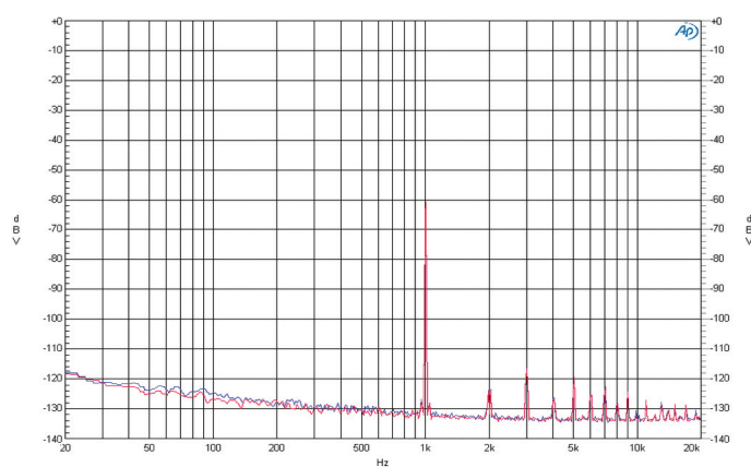
DAC playback ( Path 1) - Load 10k -60 dBFs / 1kHz Input - F_s = 48\text{kHz} - 32kpts FFT
