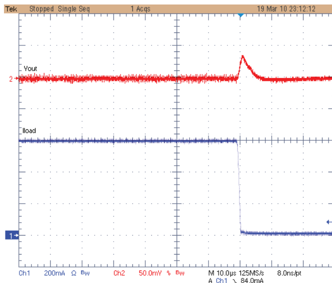
DCDC0 - VIN = 5.5V - VOUT = 1.85V Load Step 600 To 0mA / 1µs
