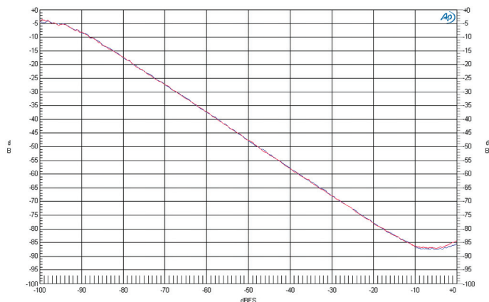
DAC playback ( Path 1) - Load 10k THD+N Ratio Versus Input Level
