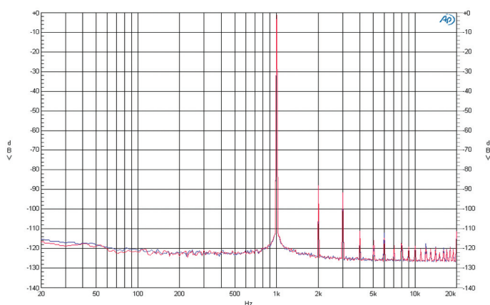
DAC playback ( Path 1) - Load 10k 0 dBFs / 1kHz Input - F_s = 48\text{kHz} - 32kpts FFT
