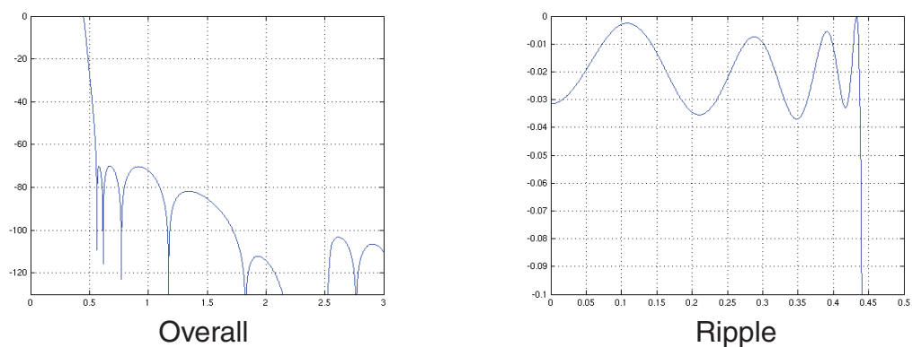
Figure 12-20. ADC Type 4 Frequency Response
