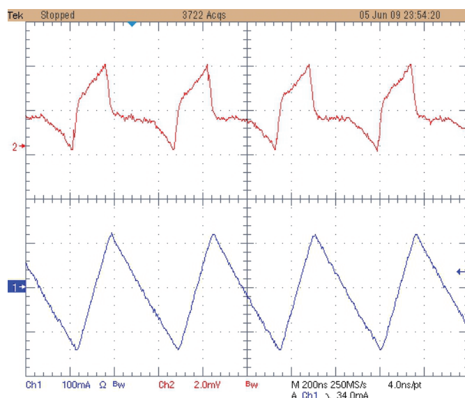
DCDC0 - VIN = 5.5V - VOUT = 1.8V Output Voltage Ripple
