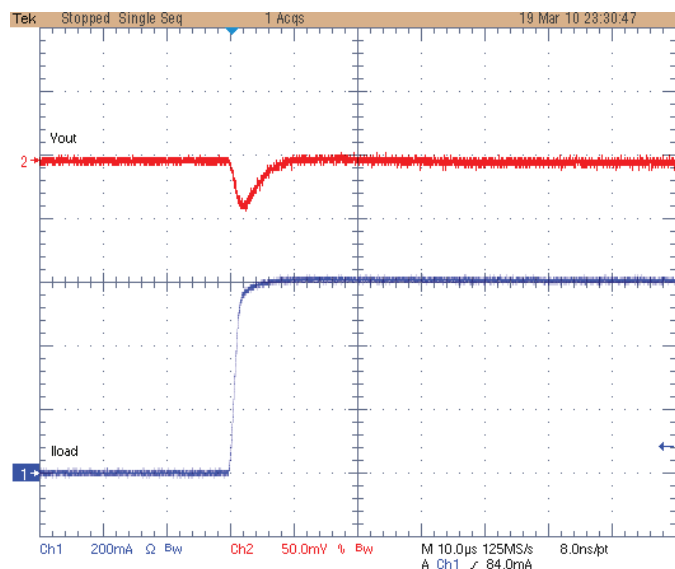
Figure 15-9. DCDC1 Transient Load Regulation Performance
