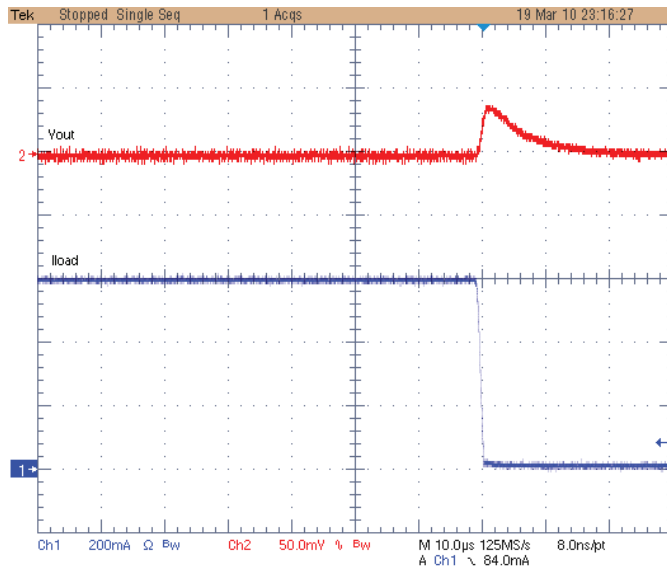
DCDC0 - VIN = 3.3V - VOUT = 1.85V Load Step 600 To 0mA / 1µs
