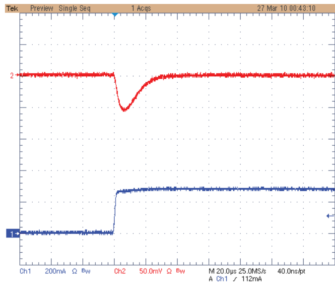
Figure 15-11. LDO2 Tansient and Static Load Regulation Performance
