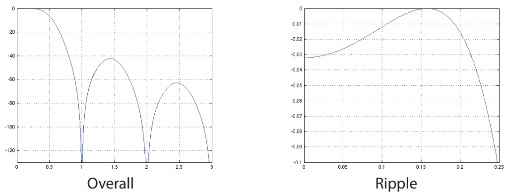
Figure 12-15. DAC Type 4 Frequency Response
