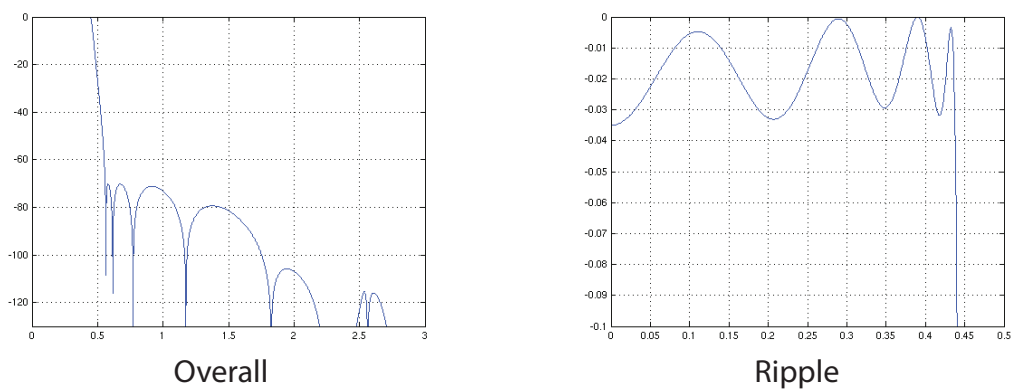
Figure 12-14. DAC Type 3 Frequency Response
