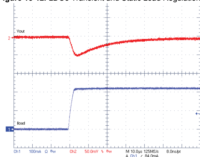
LDO3- VIN = 5.5V - VDD3 = 3.3V Load Step 0 To 200mA / 1µs
