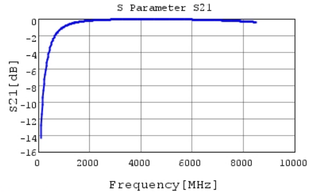
GRM1555C2A3R1WA01 S21 DCOV, 25degC
