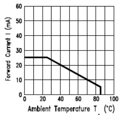
Fig.3 Forward Current A Derating Curve
