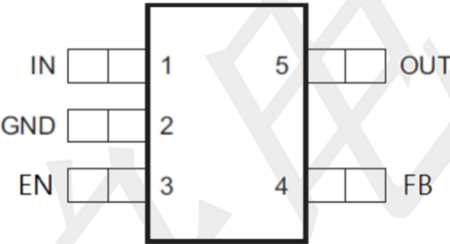
SOT23-5(TOP VIEW)
