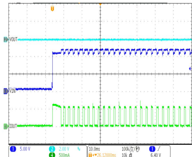
Short-circuit Power-on
